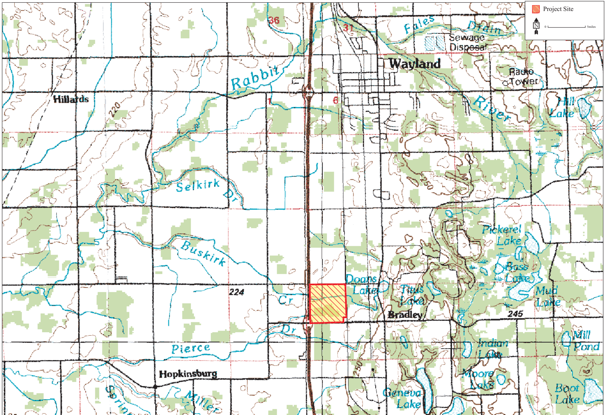
Figure 3-5 Regional Drainages
